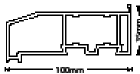
Stub cill
